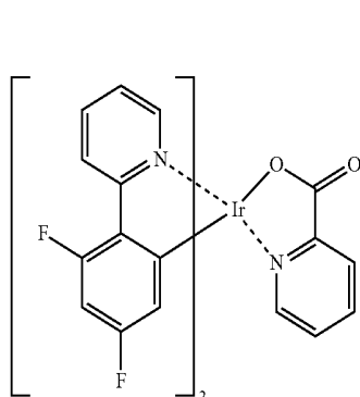
F 2 Irpic
