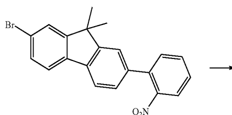
Reaction Scheme 6
