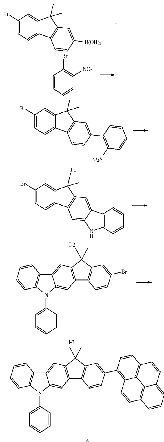
Reaction Scheme 1
