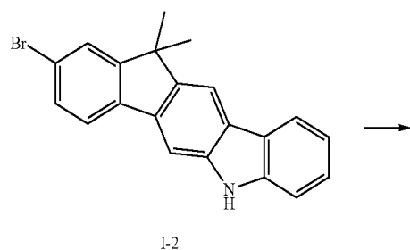
Reaction Scheme 3
