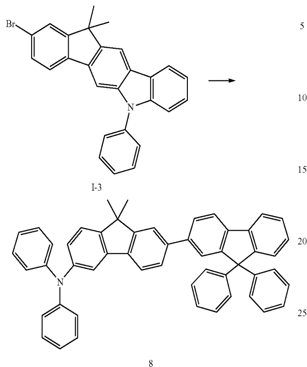
Reaction Scheme 2
